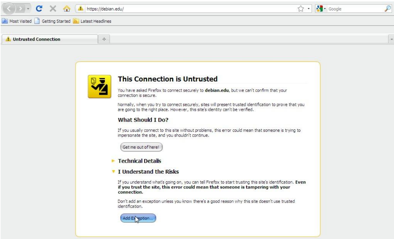
Gambar 41. Untrusted Connection
