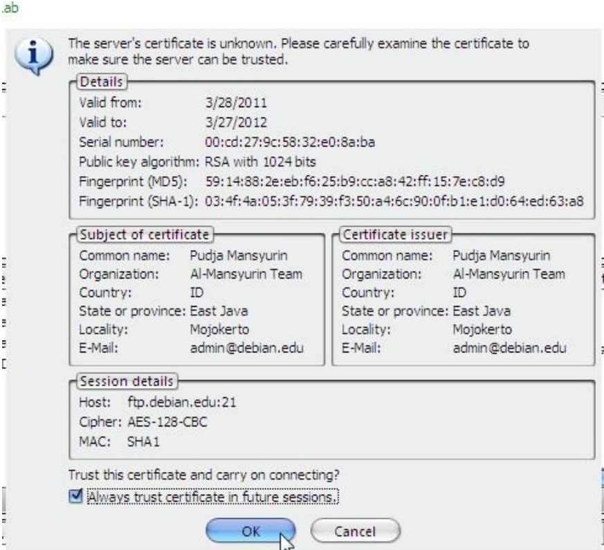
Gambar 44. FTPS Connection
