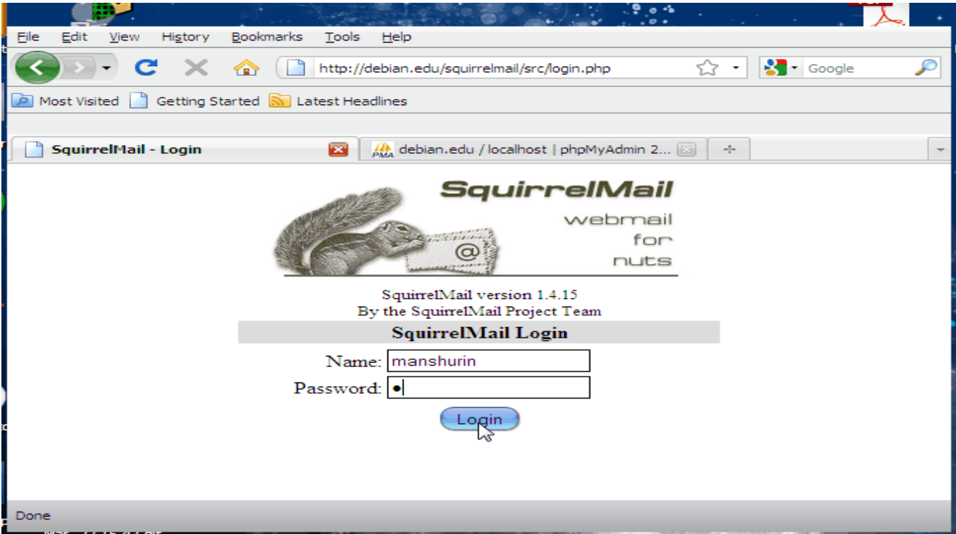
Gambar 19. Squirrel Mail
