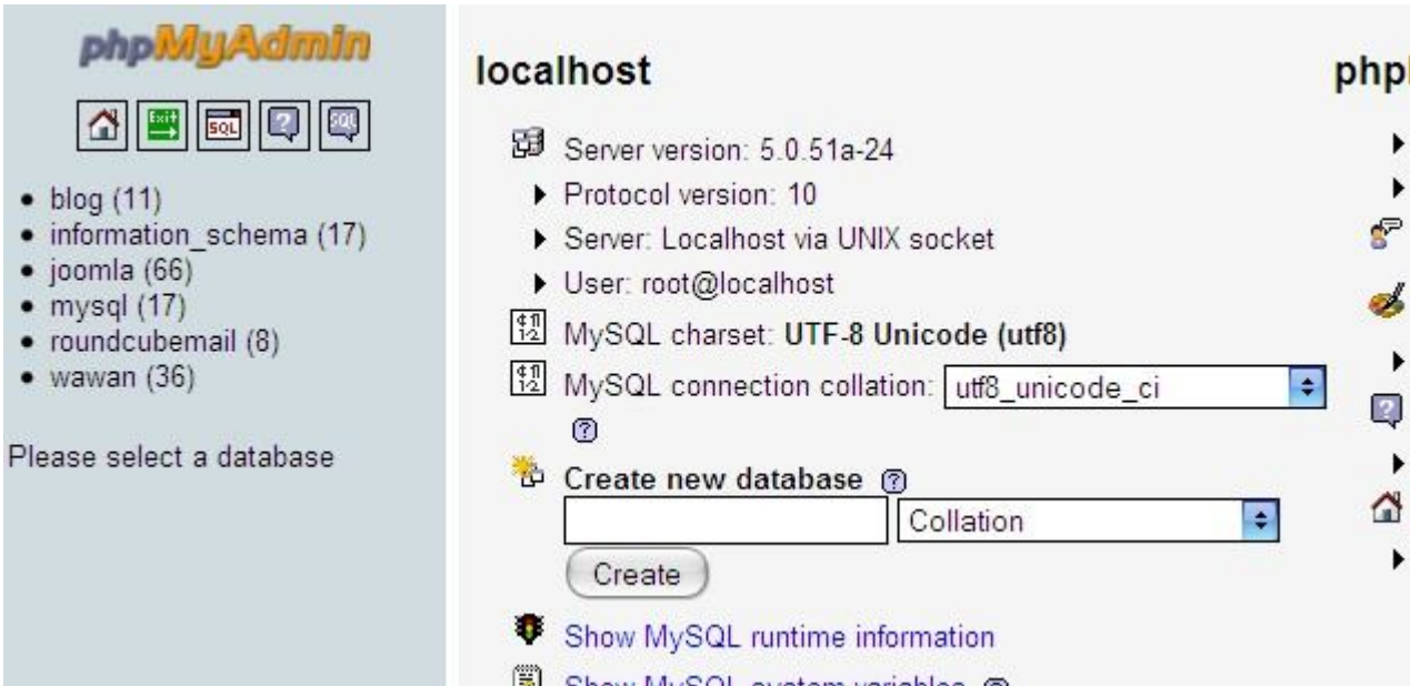
Gambar 6. Tampilan PhpMyAdmin
