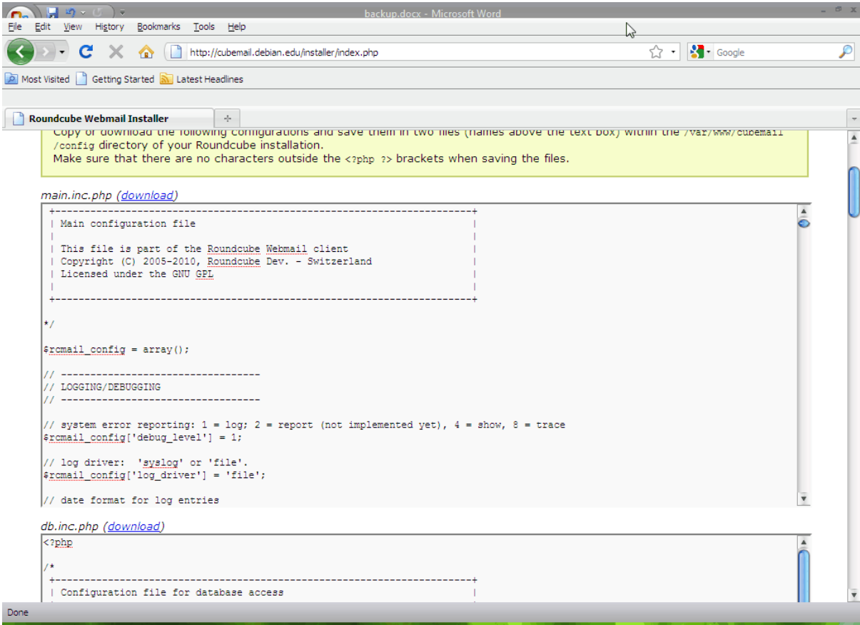
Gambar 18. File Configuration
